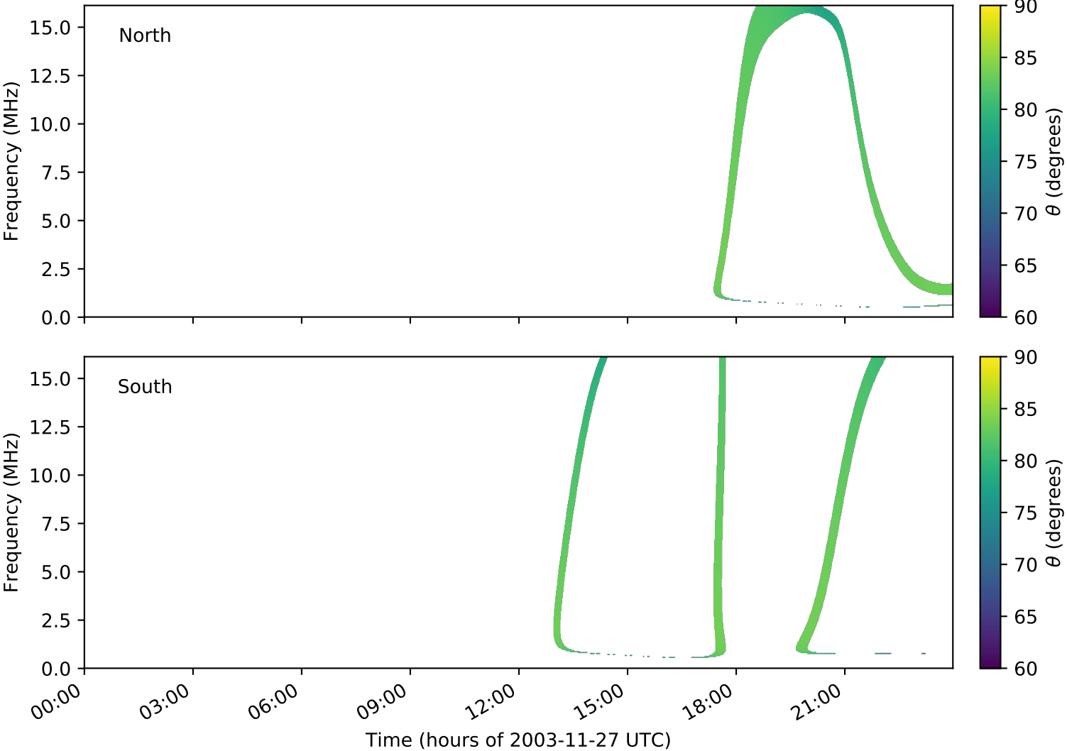
expres_cassini_jupiter_ganymede_isaac_lossc-wid1deg_3kev_20031127_v01.cdf
