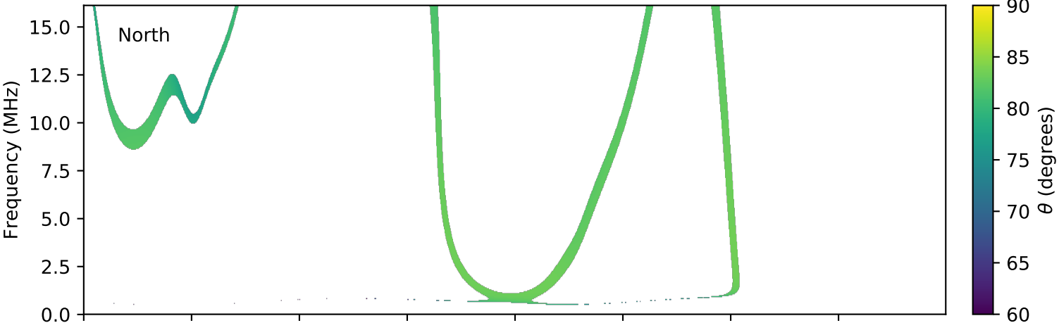
expres_cassini_jupiter_ganymede_isaac_lossc-wid1deg_3kev_20031123_v01.cdf
