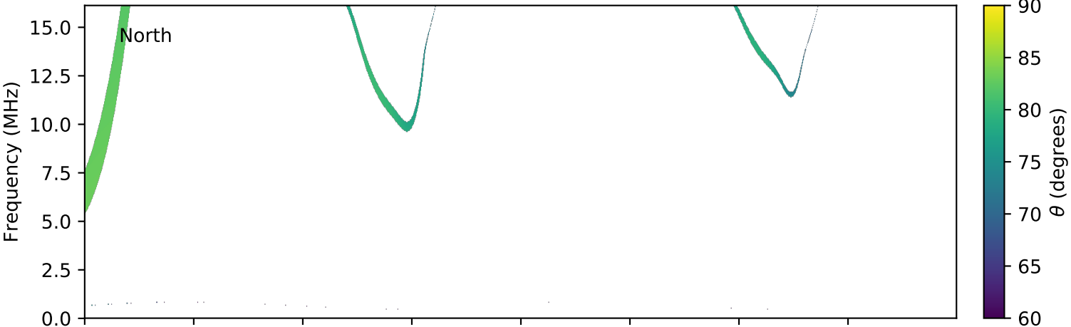
expres_cassini_jupiter_ganymede_isaac_lossc-wid1deg_3kev_20031121_v01.cdf
