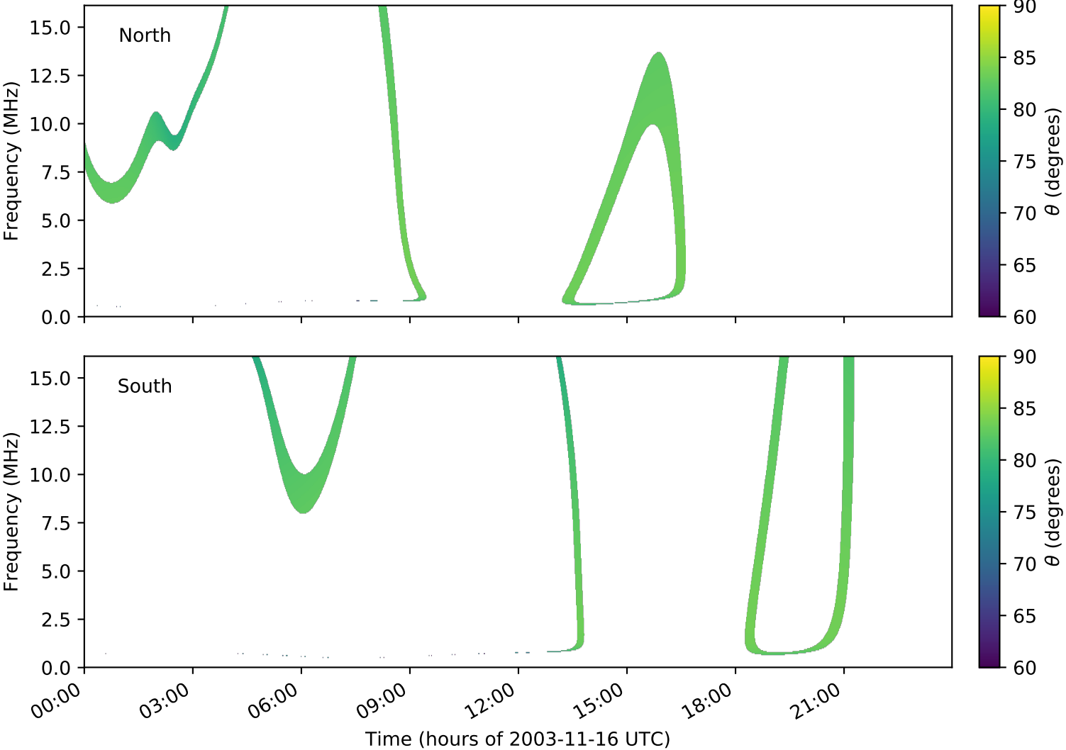
expres_cassini_jupiter_ganymede_isaac_lossc-wid1deg_3kev_20031116_v01.cdf
