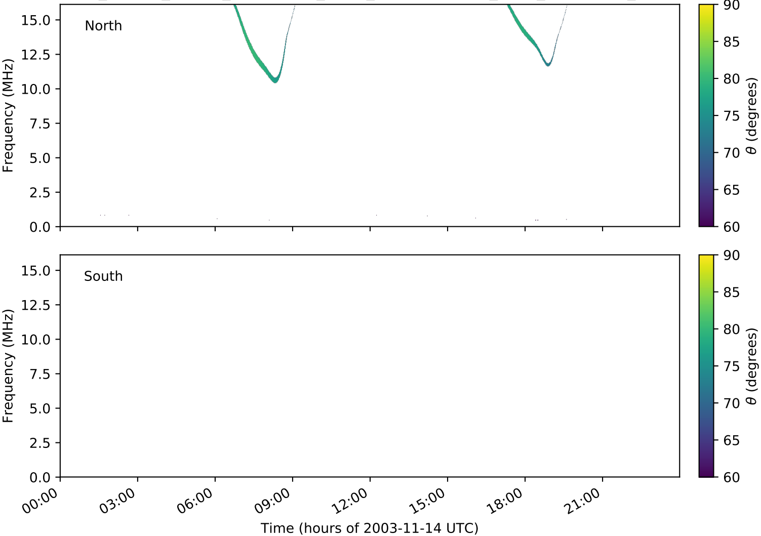
expres_cassini_jupiter_ganymede_isaac_lossc-wid1deg_3kev_20031114_v01.cdf
