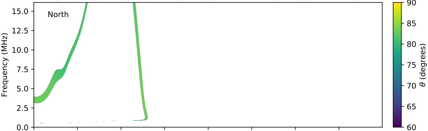
expres_cassini_jupiter_ganymede_isaac_lossc-wid1deg_3kev_20031109_v01.cdf
