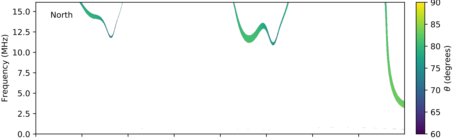
expres_cassini_jupiter_ganymede_isaac_lossc-wid1deg_3kev_20031108_v01.cdf
