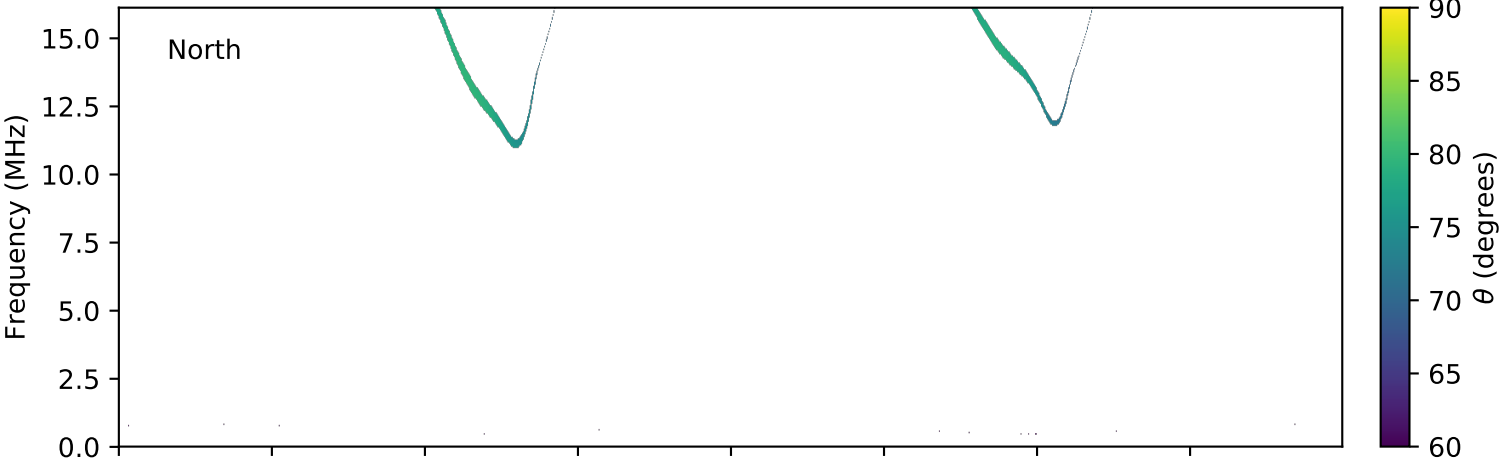
expres_cassini_jupiter_ganymede_isaac_lossc-wid1deg_3kev_20031107_v01.cdf
