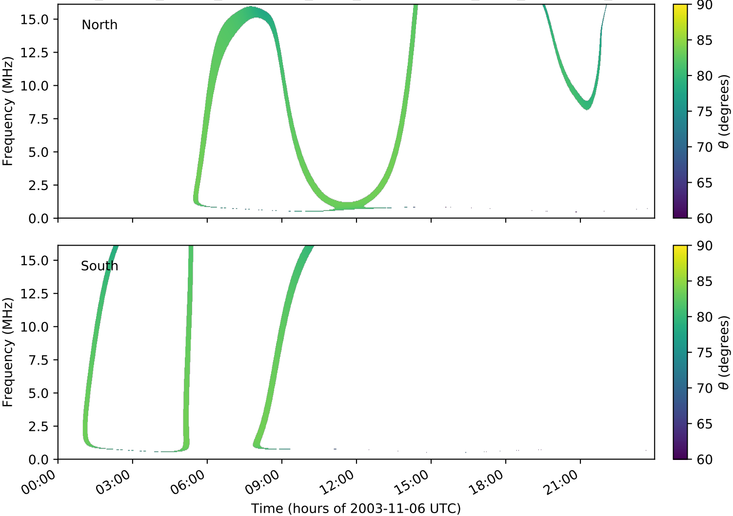
expres_cassini_jupiter_ganymede_isaac_lossc-wid1deg_3kev_20031106_v01.cdf
