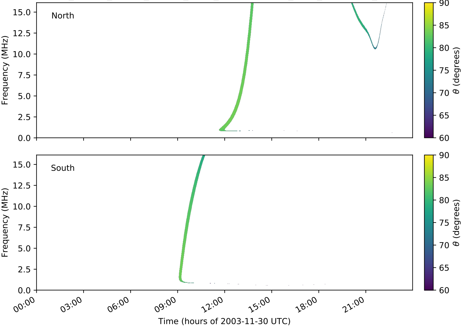
expres_cassini_jupiter_europa_isaac_lossc-wid1deg_3kev_20031130_v01.cdf
