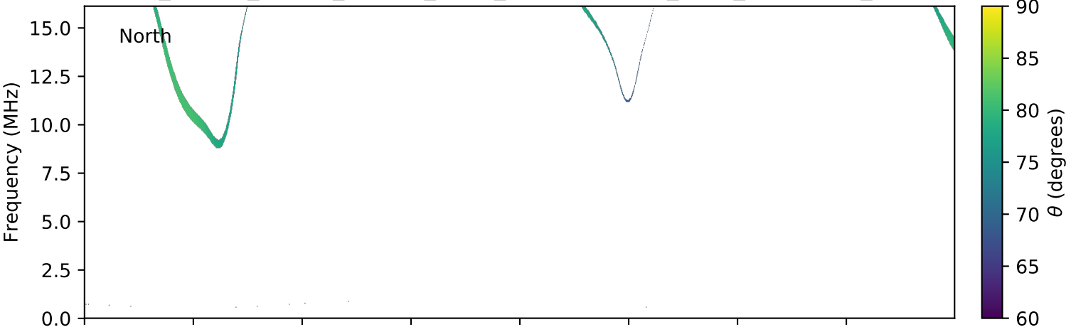
expres_cassini_jupiter_europa_isaac_lossc-wid1deg_3kev_20031127_v01.cdf
