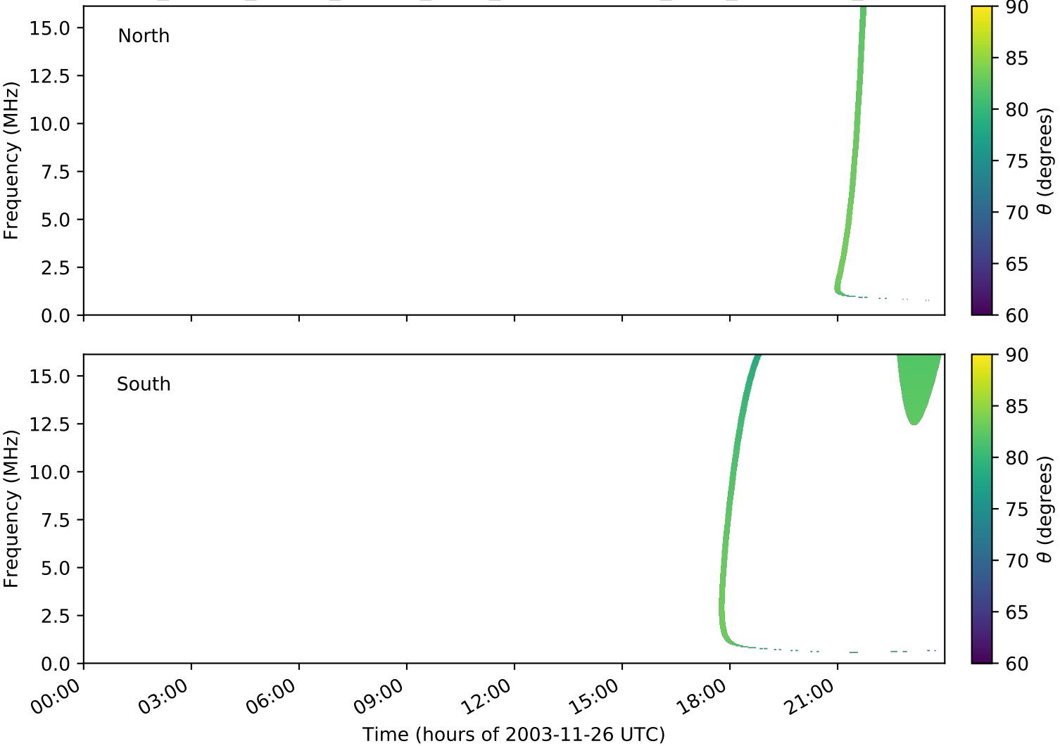
expres_cassini_jupiter_europa_isaac_lossc-wid1deg_3kev_20031126_v01.cdf
