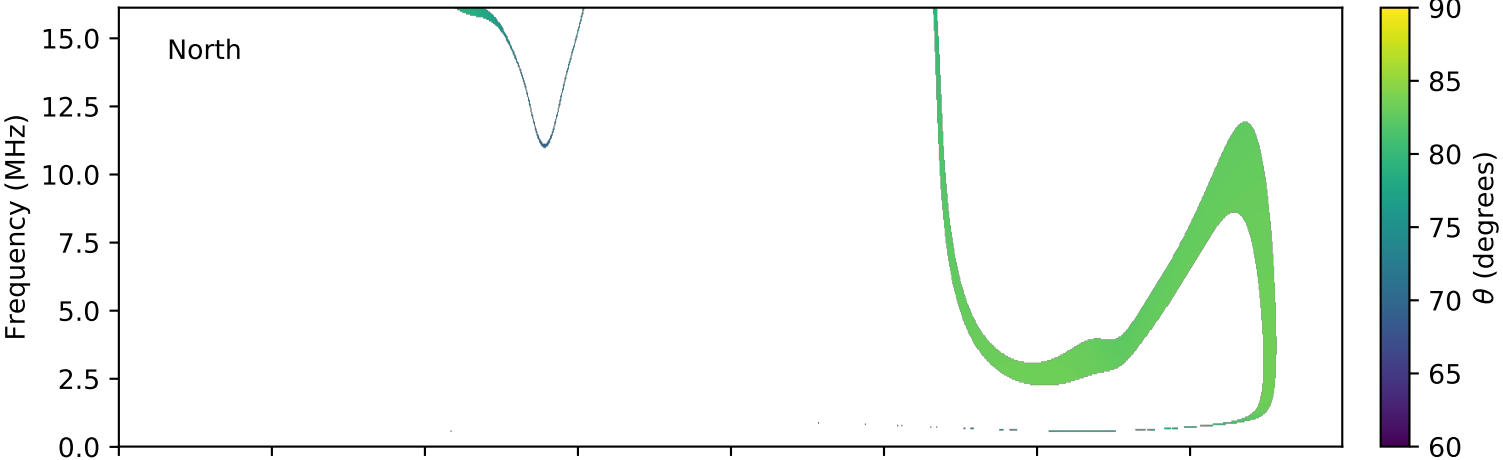
expres_cassini_jupiter_europa_isaac_lossc-wid1deg_3kev_20031124_v01.cdf
