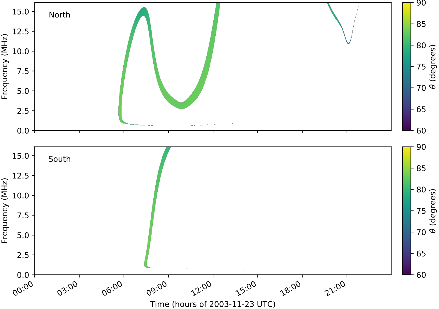
expres_cassini_jupiter_europa_isaac_lossc-wid1deg_3kev_20031123_v01.cdf
