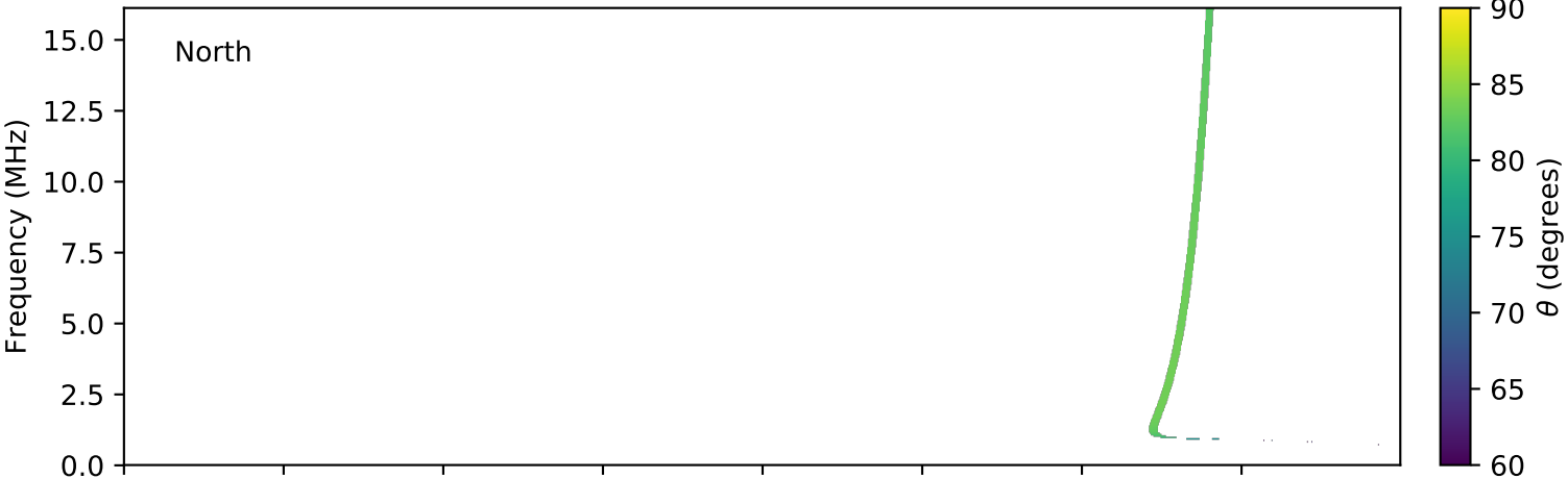
expres_cassini_jupiter_europa_isaac_lossc-wid1deg_3kev_20031119_v01.cdf
