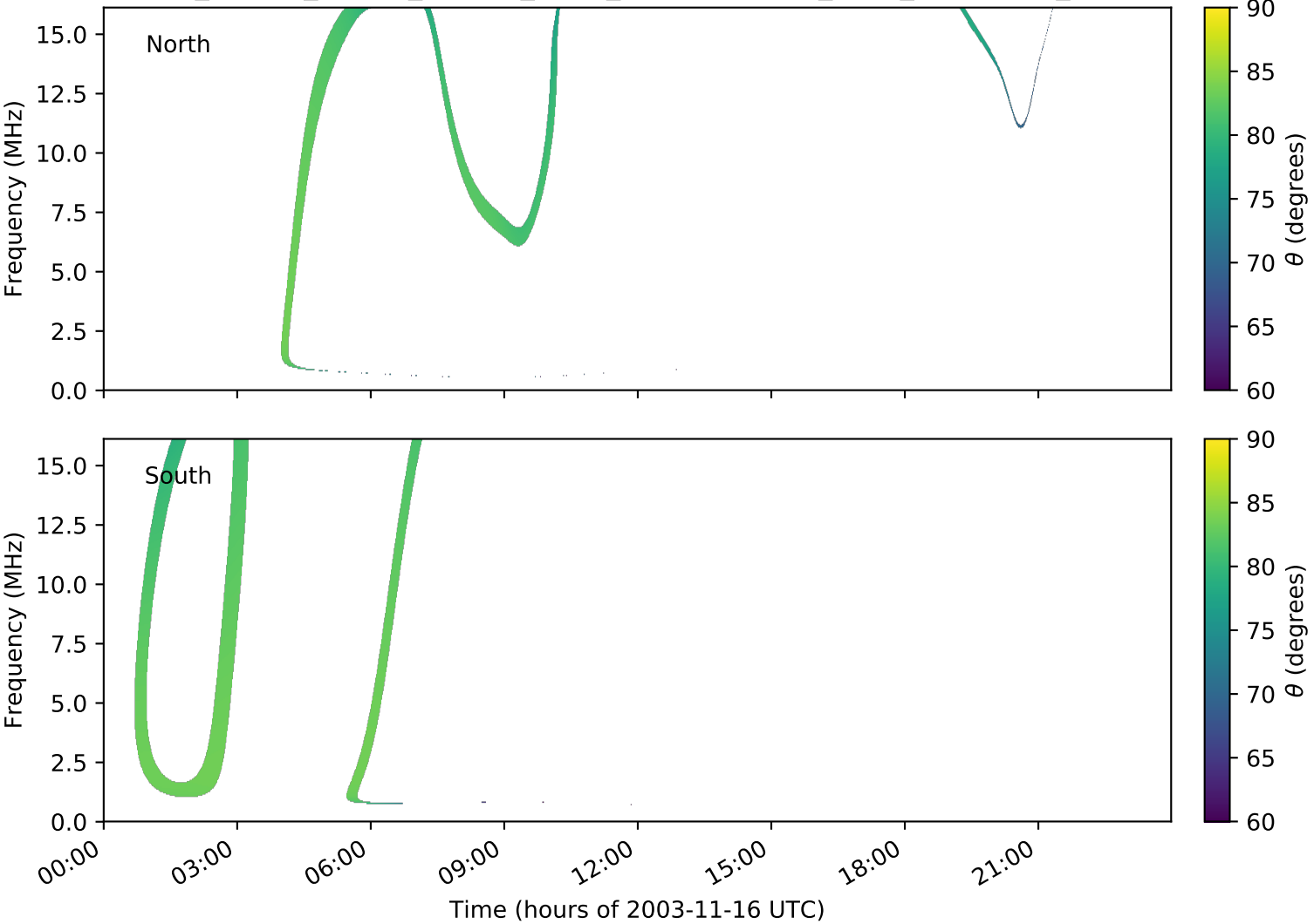
expres_cassini_jupiter_europa_isaac_lossc-wid1deg_3kev_20031116_v01.cdf
