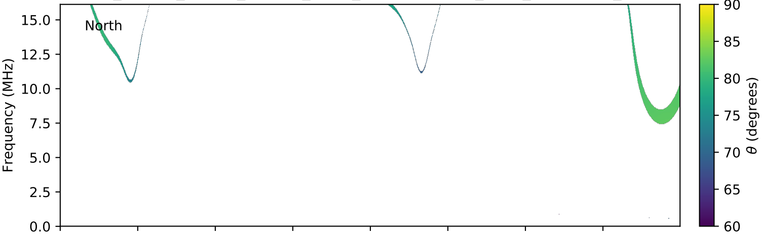
expres_cassini_jupiter_europa_isaac_lossc-wid1deg_3kev_20031113_v01.cdf
