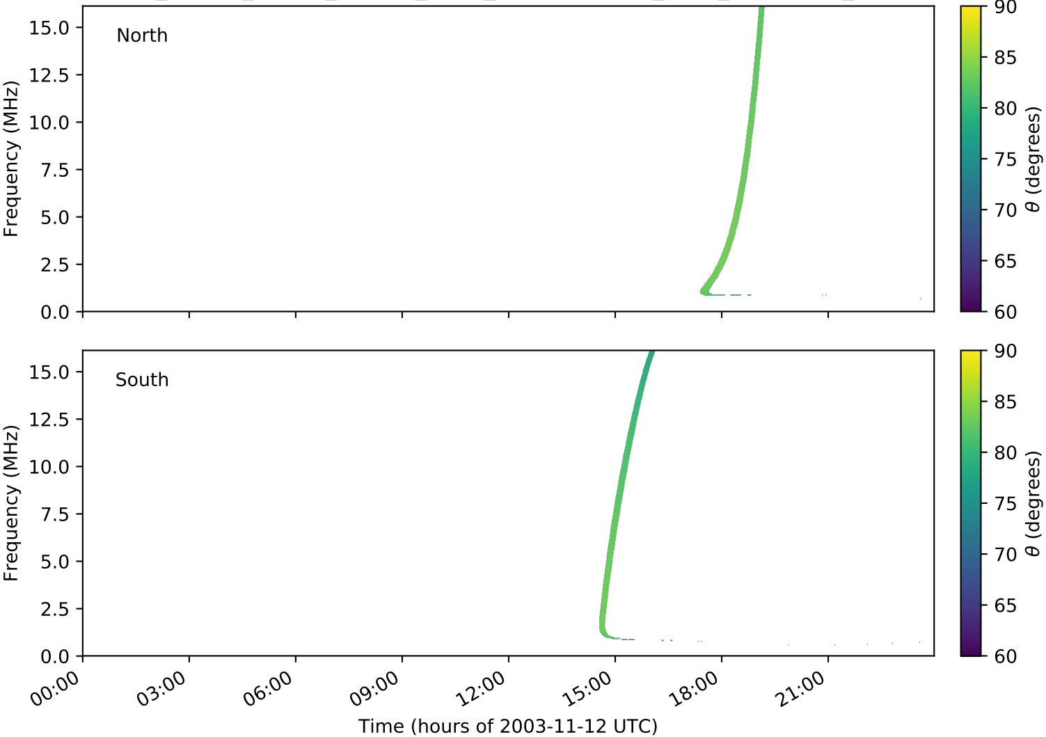
expres_cassini_jupiter_europa_isaac_lossc-wid1deg_3kev_20031112_v01.cdf
