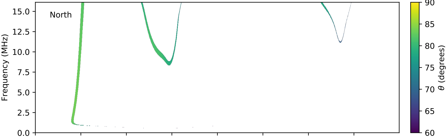
expres_cassini_jupiter_europa_isaac_lossc-wid1deg_3kev_20031109_v01.cdf
