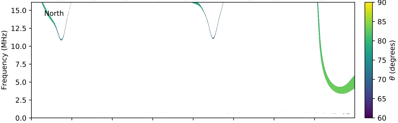
expres_cassini_jupiter_europa_isaac_lossc-wid1deg_3kev_20031106_v01.cdf
