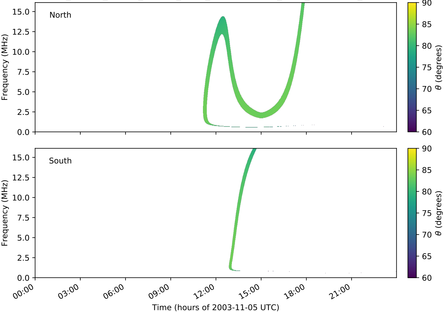
expres_cassini_jupiter_europa_isaac_lossc-wid1deg_3kev_20031105_v01.cdf
