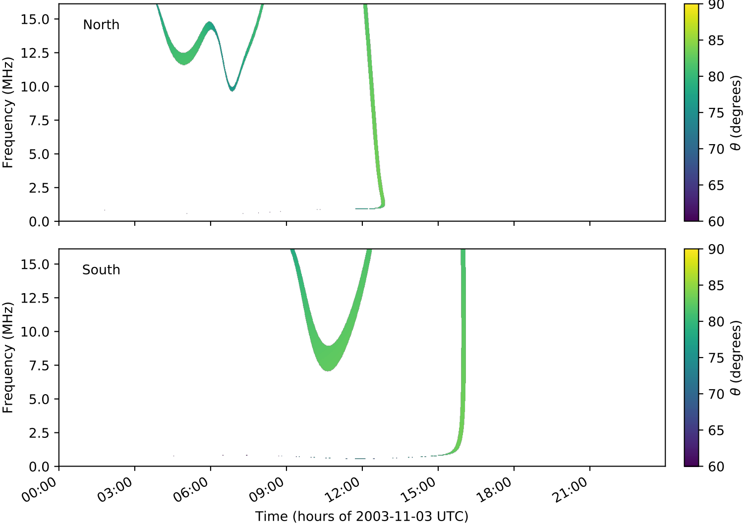
expres_cassini_jupiter_europa_isaac_lossc-wid1deg_3kev_20031103_v01.cdf
