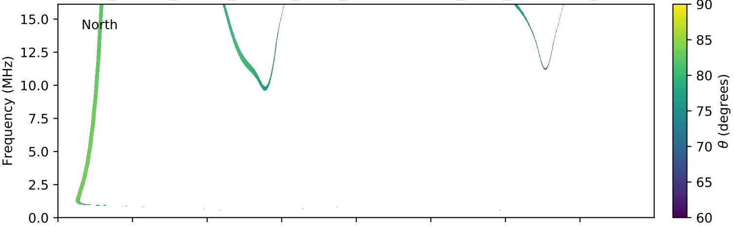
expres_cassini_jupiter_europa_isaac_lossc-wid1deg_3kev_20031102_v01.cdf
