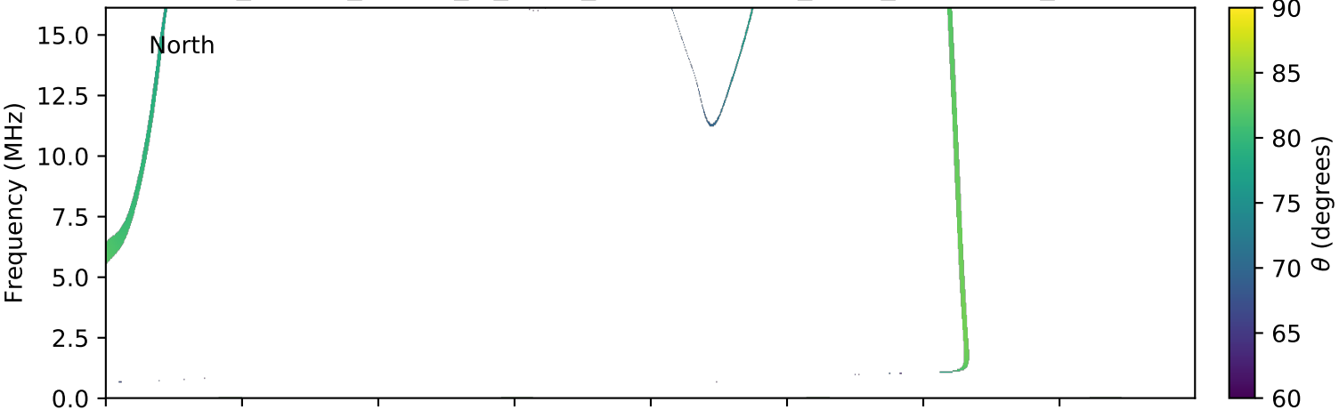
expres_cassini_jupiter_io_isaac_lossc-wid1deg_3kev_20031030_v01.cdf
