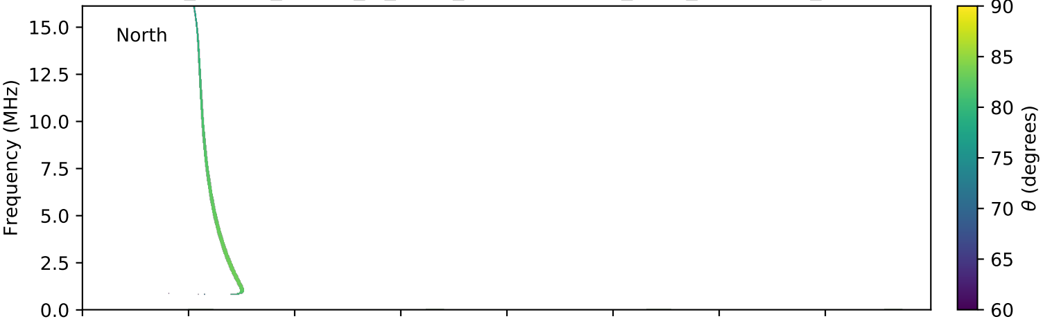
expres_cassini_jupiter_io_isaac_lossc-wid1deg_3kev_20031027_v01.cdf
