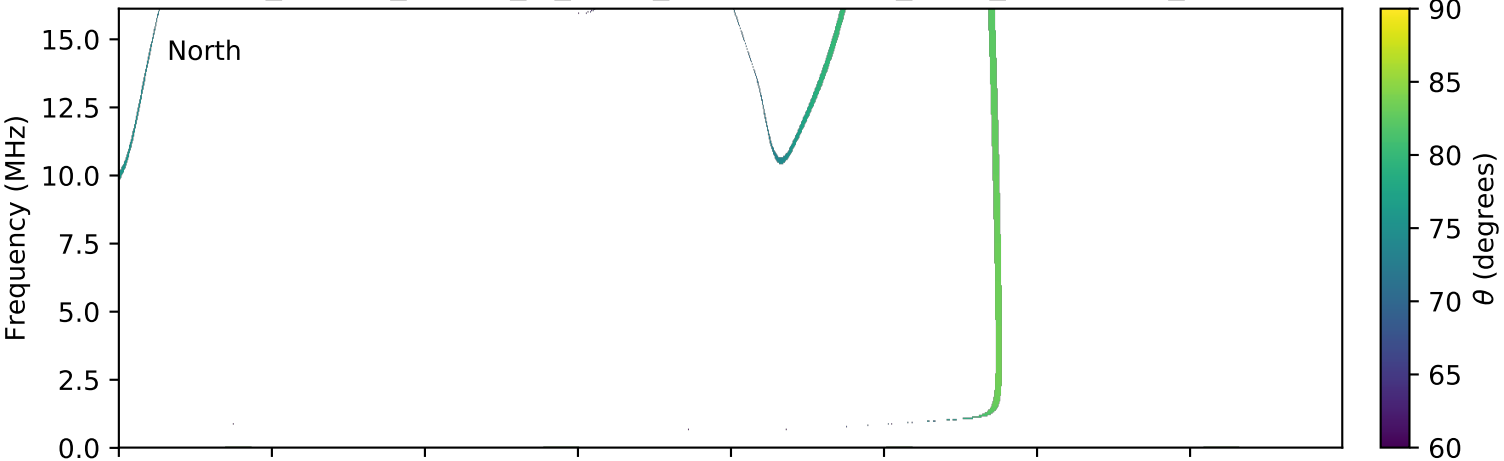
expres_cassini_jupiter_io_isaac_lossc-wid1deg_3kev_20031023_v01.cdf
