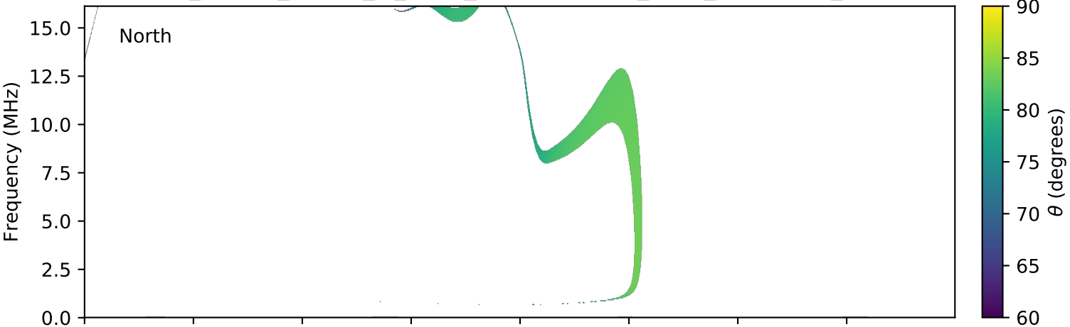
expres_cassini_jupiter_io_isaac_lossc-wid1deg_3kev_20031016_v01.cdf
