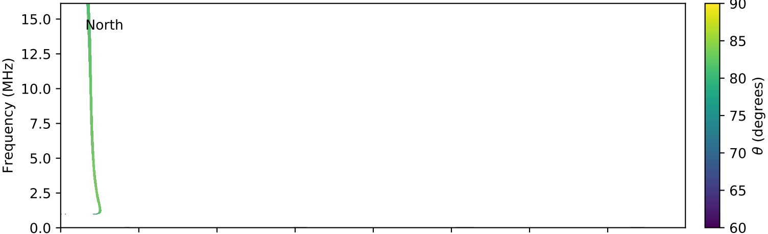
expres_cassini_jupiter_io_isaac_lossc-wid1deg_3kev_20031013_v01.cdf
