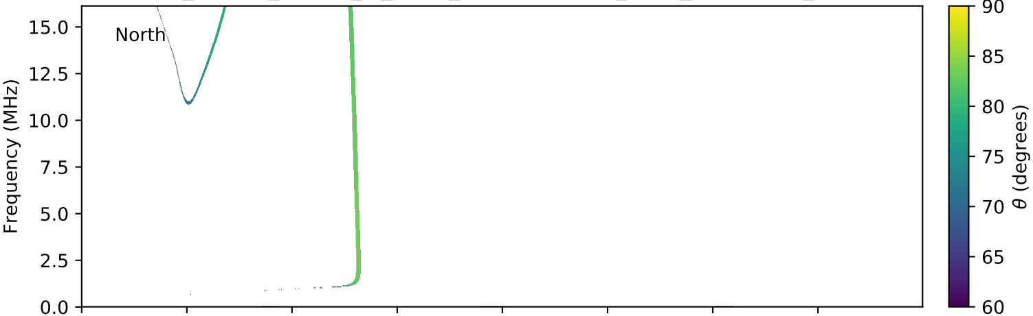
expres_cassini_jupiter_io_isaac_lossc-wid1deg_3kev_20031011_v01.cdf
