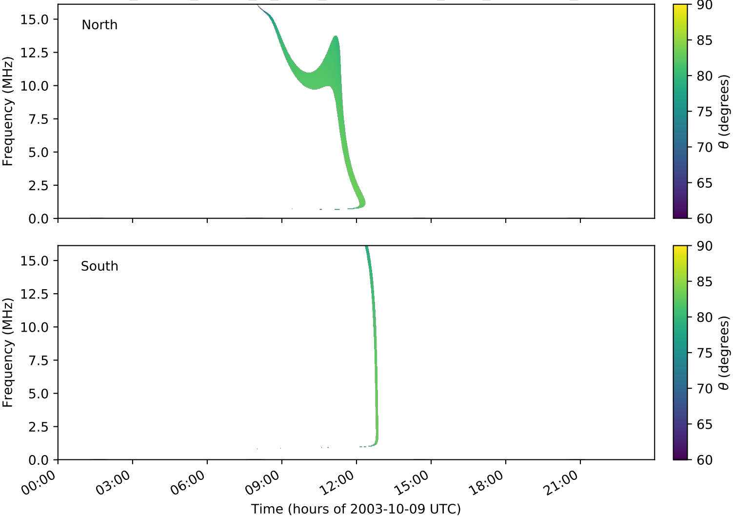
expres_cassini_jupiter_io_isaac_lossc-wid1deg_3kev_20031009_v01.cdf
