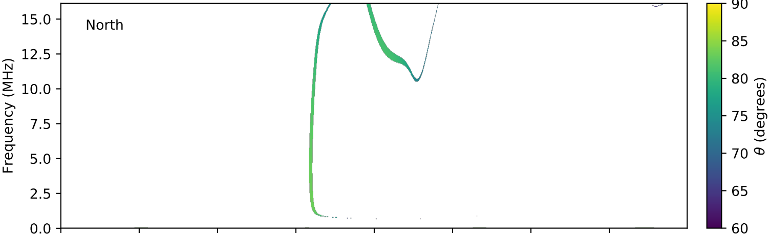
expres_cassini_jupiter_io_isaac_lossc-wid1deg_3kev_20031003_v01.cdf
