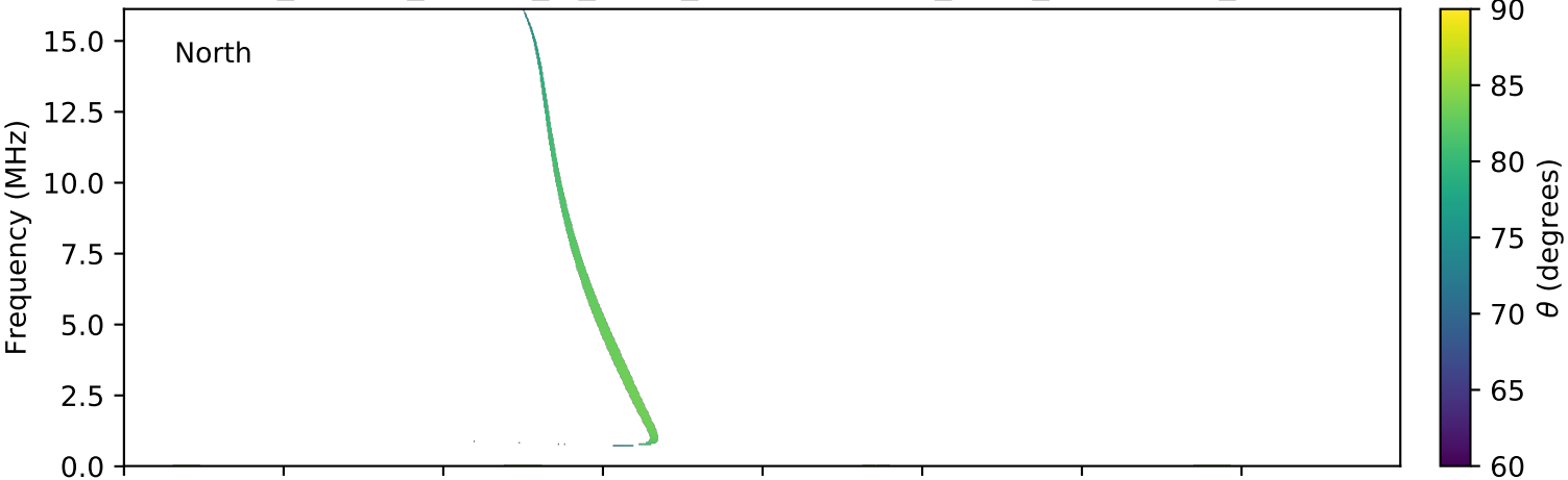
expres_cassini_jupiter_io_isaac_lossc-wid1deg_3kev_20031002_v01.cdf
