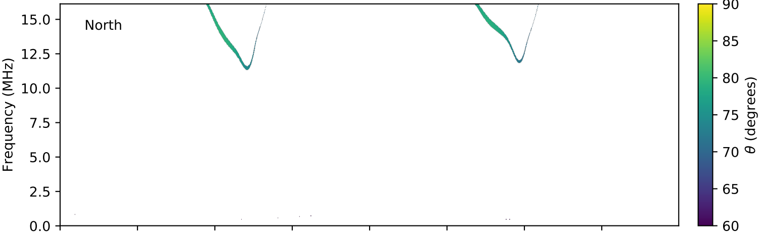
expres_cassini_jupiter_ganymede_isaac_lossc-wid1deg_3kev_20031031_v01.cdf
