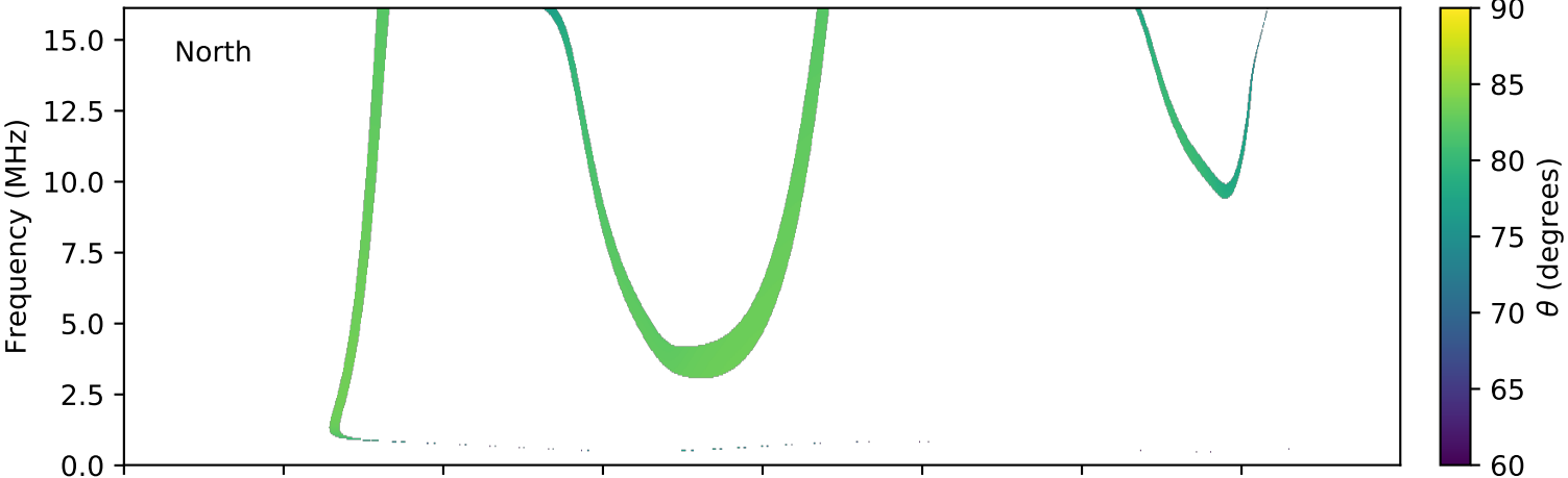
expres_cassini_jupiter_ganymede_isaac_lossc-wid1deg_3kev_20031030_v01.cdf
