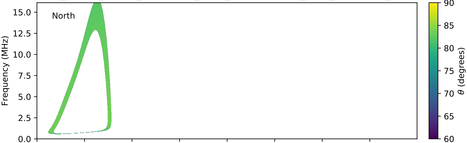
expres_cassini_jupiter_ganymede_isaac_lossc-wid1deg_3kev_20031026_v01.cdf
