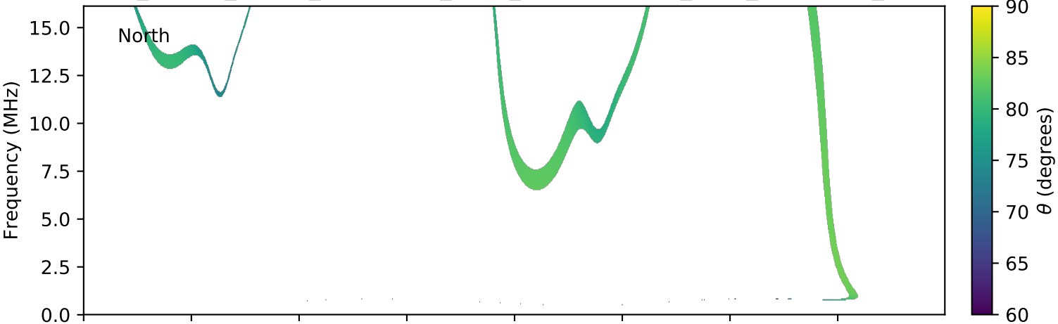
expres_cassini_jupiter_ganymede_isaac_lossc-wid1deg_3kev_20031025_v01.cdf
