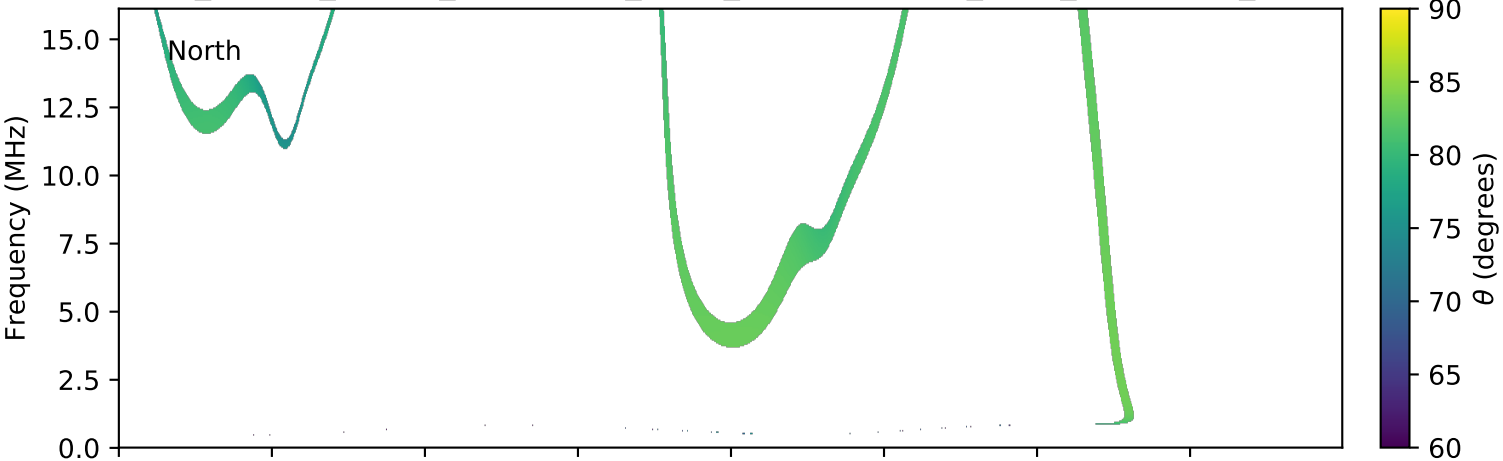
expres_cassini_jupiter_ganymede_isaac_lossc-wid1deg_3kev_20031018_v01.cdf
