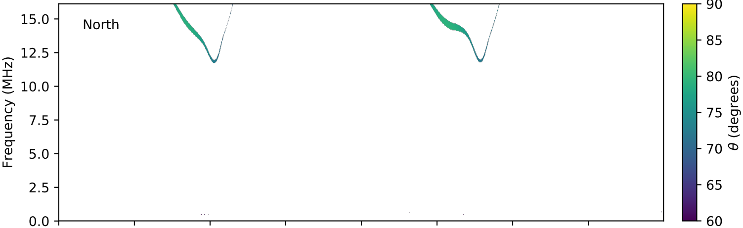
expres_cassini_jupiter_ganymede_isaac_lossc-wid1deg_3kev_20031017_v01.cdf
