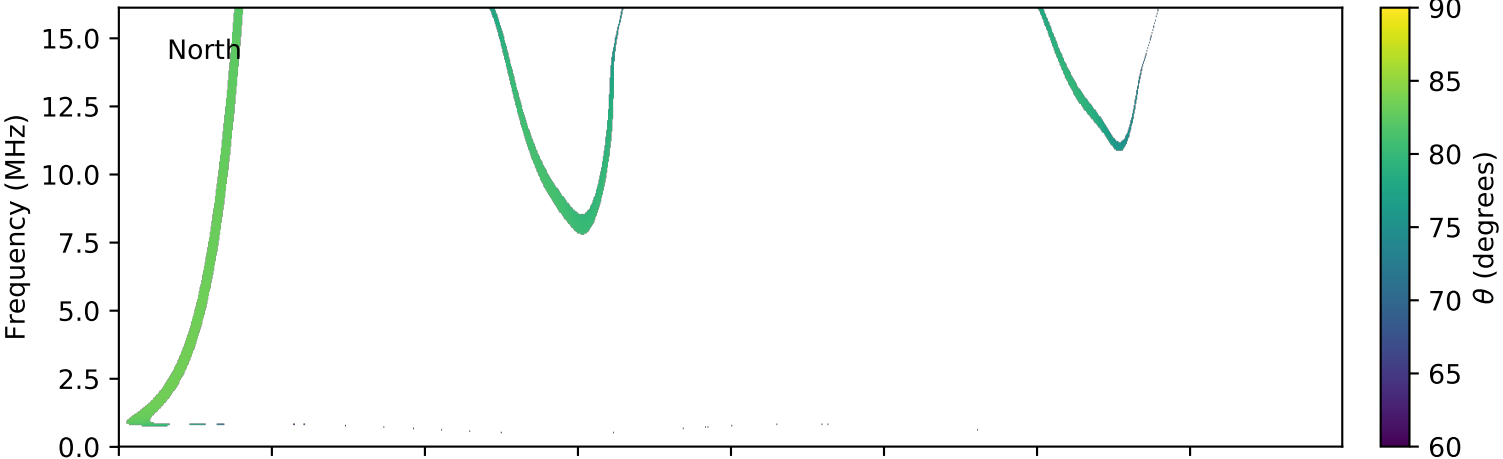
expres_cassini_jupiter_ganymede_isaac_lossc-wid1deg_3kev_20031016_v01.cdf
