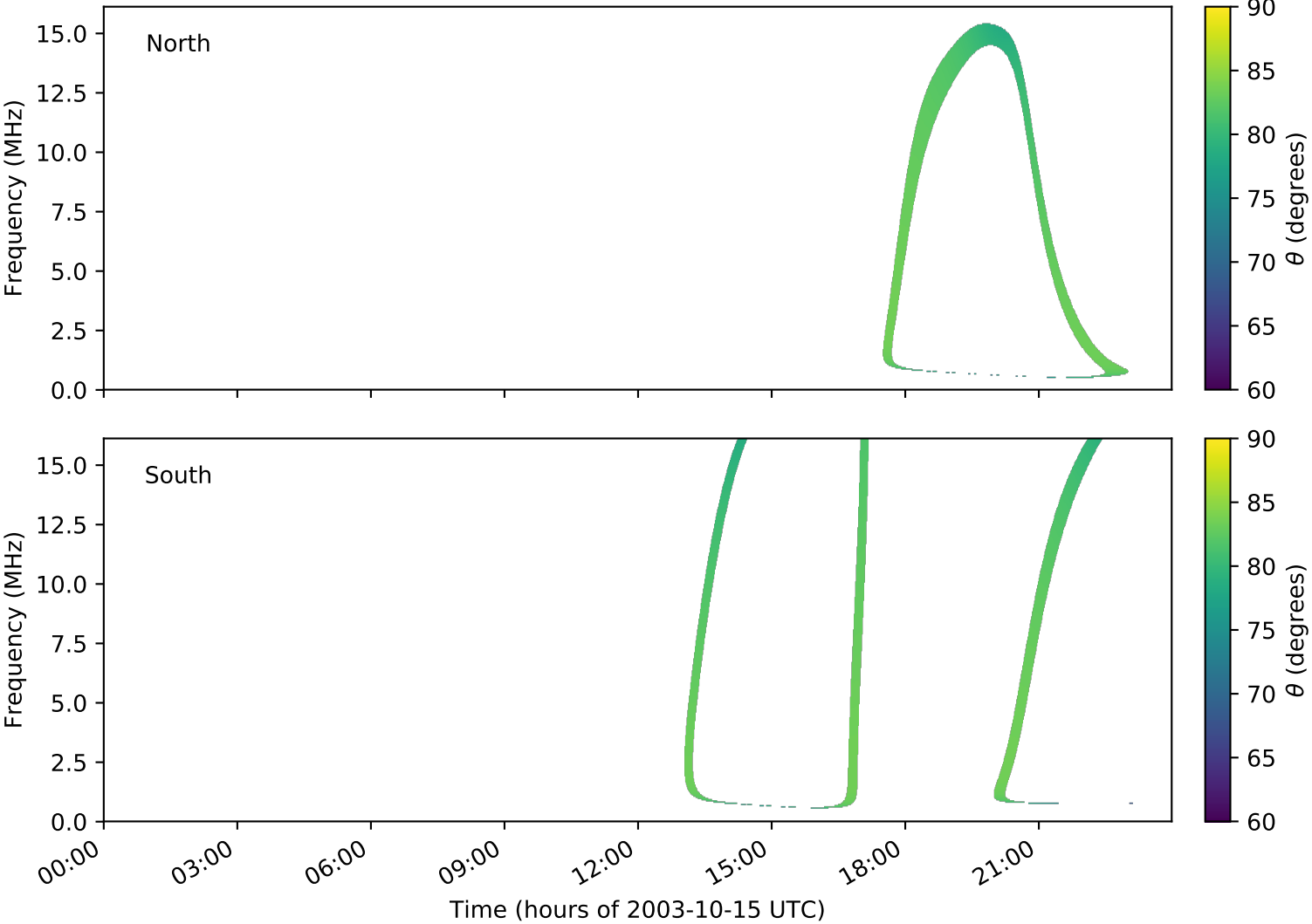
expres_cassini_jupiter_ganymede_isaac_lossc-wid1deg_3kev_20031015_v01.cdf
