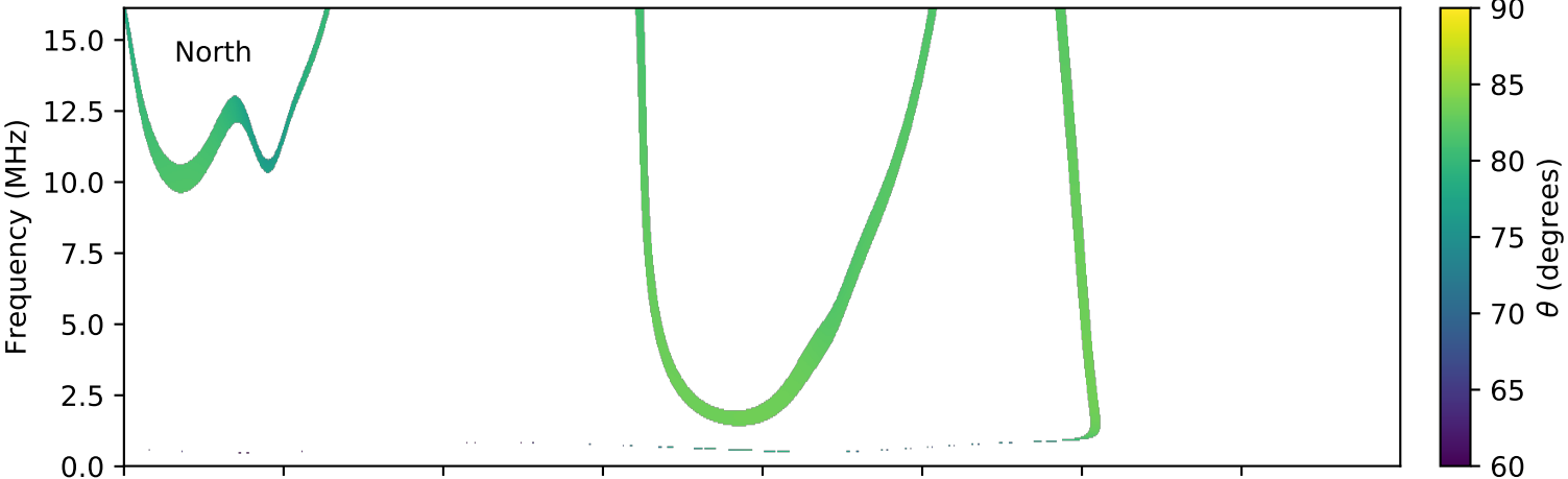
expres_cassini_jupiter_ganymede_isaac_lossc-wid1deg_3kev_20031011_v01.cdf
