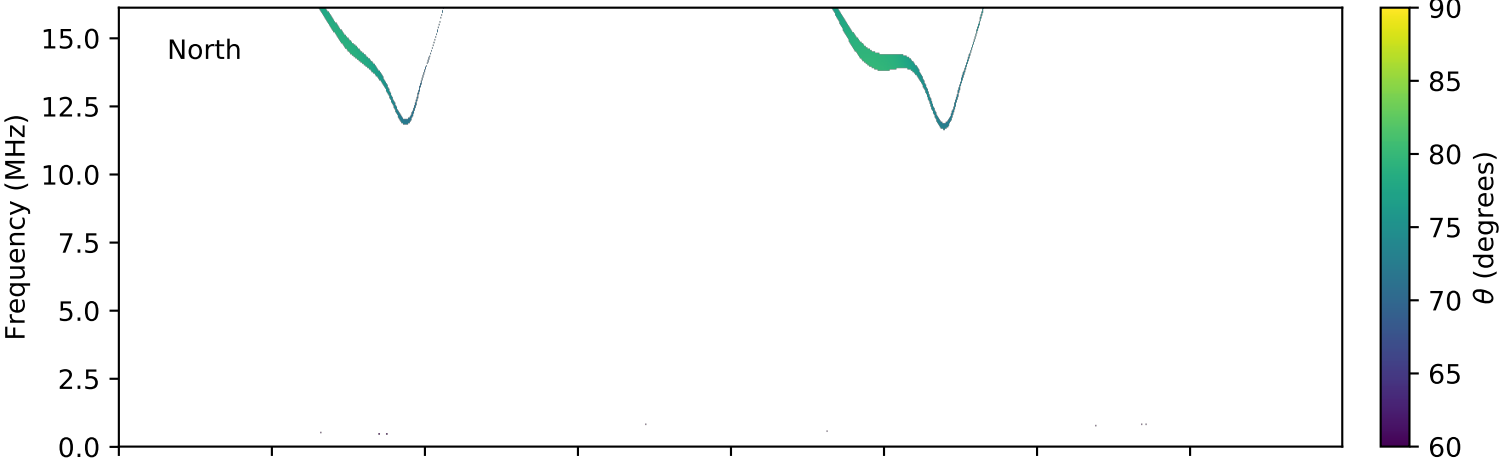
expres_cassini_jupiter_ganymede_isaac_lossc-wid1deg_3kev_20031010_v01.cdf
