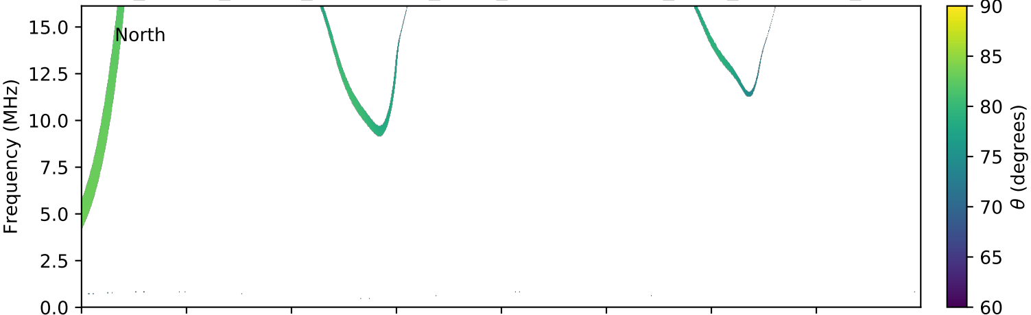
expres_cassini_jupiter_ganymede_isaac_lossc-wid1deg_3kev_20031009_v01.cdf
