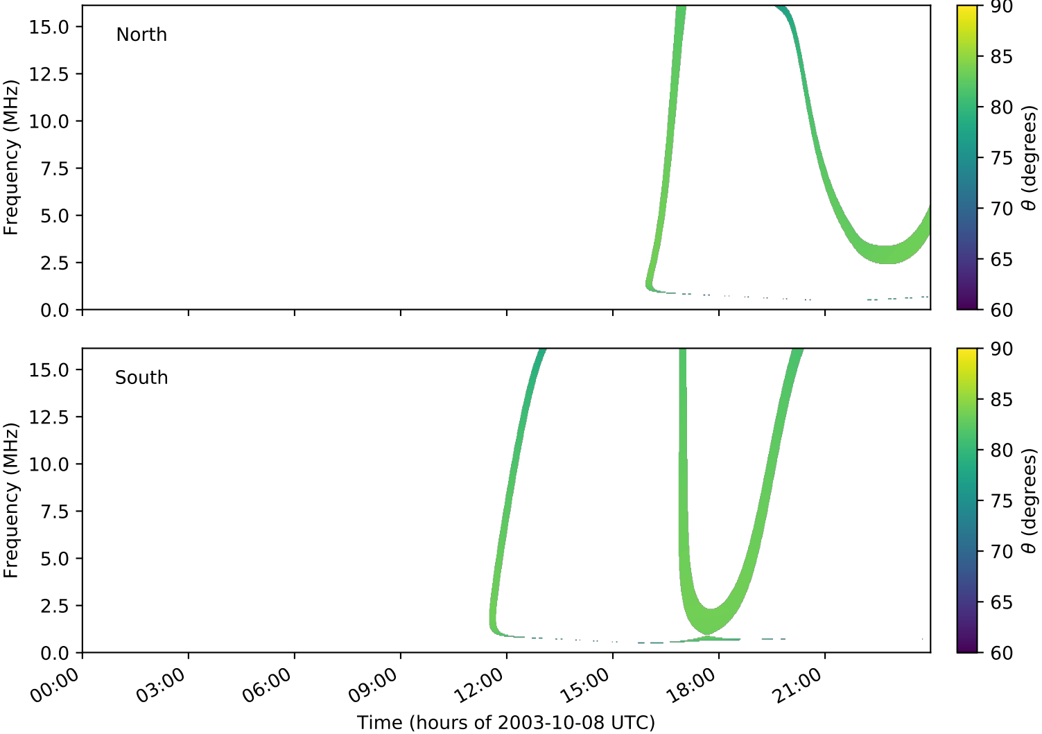
expres_cassini_jupiter_ganymede_isaac_lossc-wid1deg_3kev_20031008_v01.cdf
