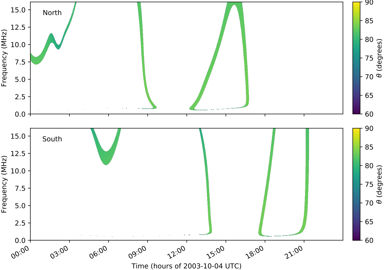
expres_cassini_jupiter_ganymede_isaac_lossc-wid1deg_3kev_20031004_v01.cdf
