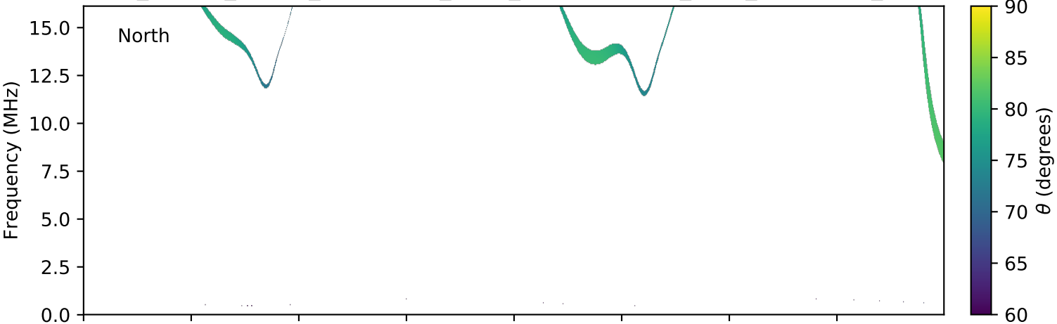
expres_cassini_jupiter_ganymede_isaac_lossc-wid1deg_3kev_20031003_v01.cdf
