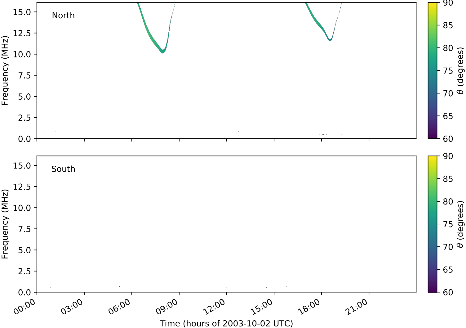
expres_cassini_jupiter_ganymede_isaac_lossc-wid1deg_3kev_20031002_v01.cdf
