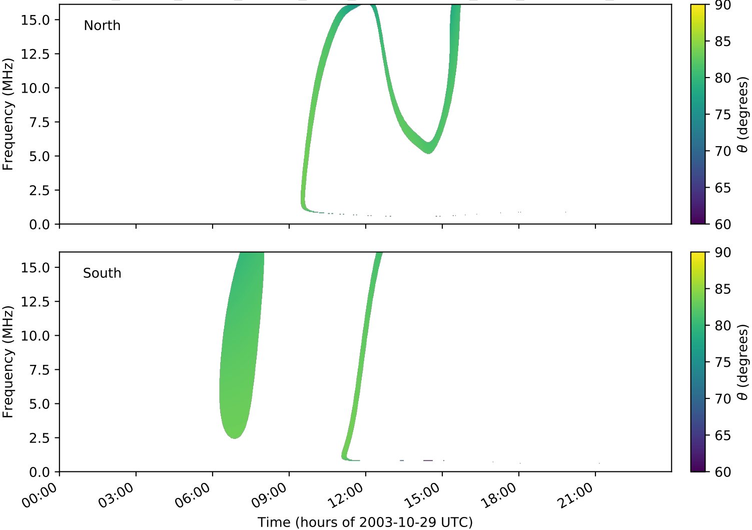
expres_cassini_jupiter_europa_isaac_lossc-wid1deg_3kev_20031029_v01.cdf
