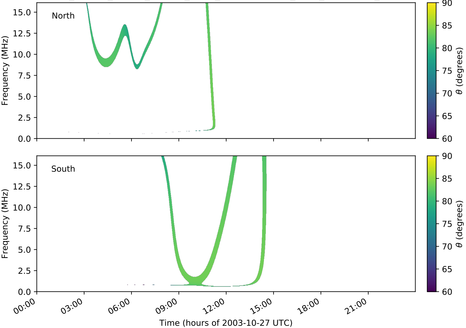
expres_cassini_jupiter_europa_isaac_lossc-wid1deg_3kev_20031027_v01.cdf
