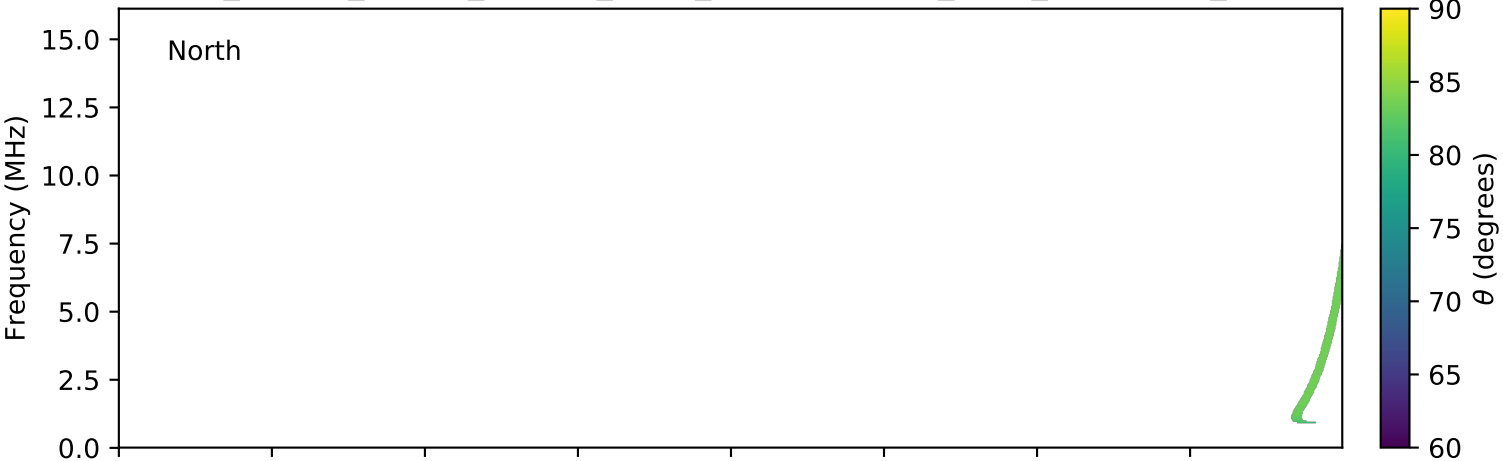
expres_cassini_jupiter_europa_isaac_lossc-wid1deg_3kev_20031025_v01.cdf
